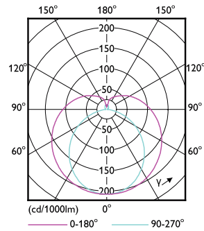
Light Distribution Diagram - MAS LEDtube 1200mm HO 14W830 T8
