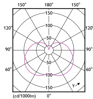
Light Distribution Diagram - LED PLC 9W 865 2P G24d
