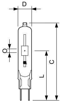
MASTERC colour CDM-TC 35W/830 G8.5 1CT/12
